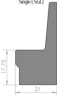
Single (-SGL)
